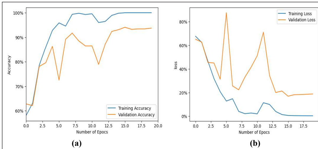
Fig. 9: (a) Accuracy (in %age) Versus Number Of Epochs Plot; (b) Loss (in %age) Versus Number of Epochs Plot for HPF-2 Hz
