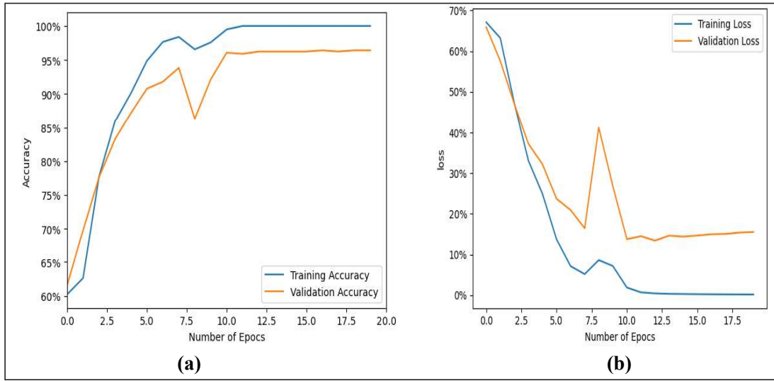
Fig. 8: (a) Accuracy (in %age) Versus Number of Epochs Plot; (b) Loss (in %age) Versus Number of Epochs Plot for HPF-1 Hz
