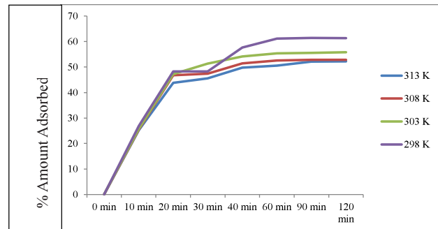
Fig. 2: Influence of Temperature on the Adsorption of Pb(II) Ions on Aluminium (III) Oxide Powder
