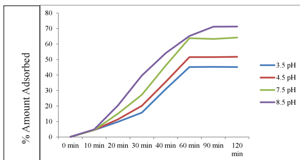
Fig. 3: Influence of pH on the Adsorption of Pb(II) Ions on Aluminium (III) Oxide Powder
